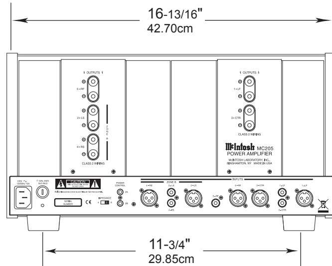
Rear View of the MC205
