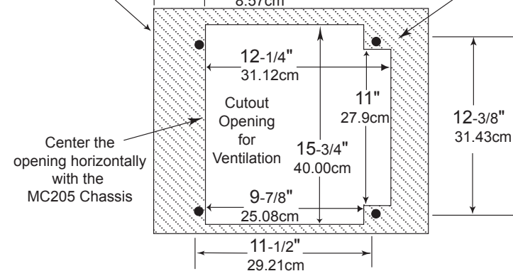
MC205 Bottom View in Custom Cabinet
