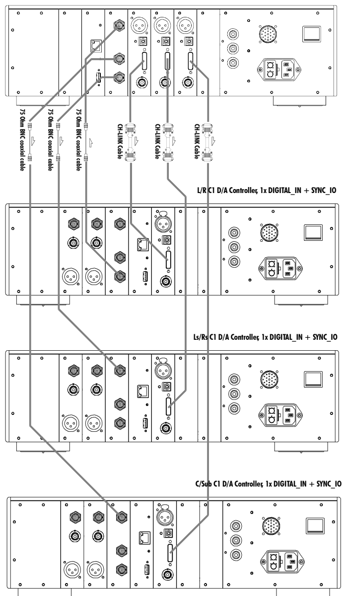
D1 SACD/CD Drive, 3x DIGITAL_OUT (L/R + Ls/Rs + C/Sub) + SYNC_IO
