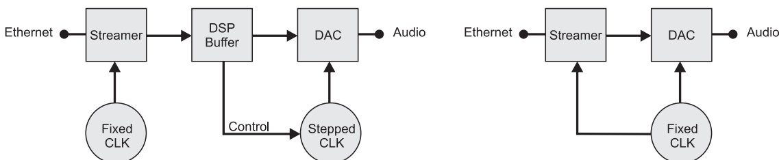
Figure 2. Old (left) and new (right) methods of controlling data flow from the network
