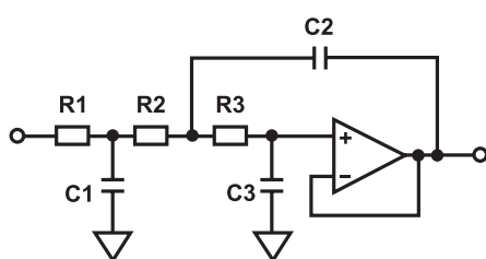
Figure 8. Circuit configuration of a Sallen and Key third-order low-pass filter
