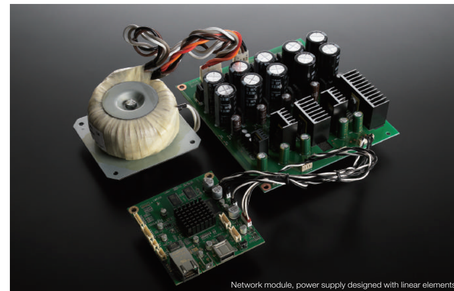
Network module, power supply designed with linear elements.
