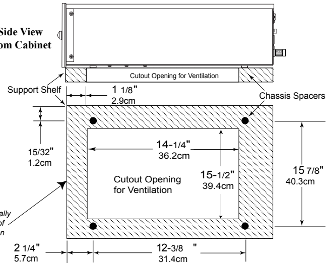
MI347 Bottom View in Custom Cabinet
