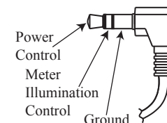
Figure 10– Mini plug for Power Control (Trigger)
