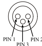
Figure 02– XLR pin diagram
