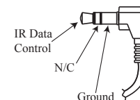
Figure 05– IR 3.5mm connector
