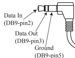
Figure 03– Mini plug for RS232 connection
