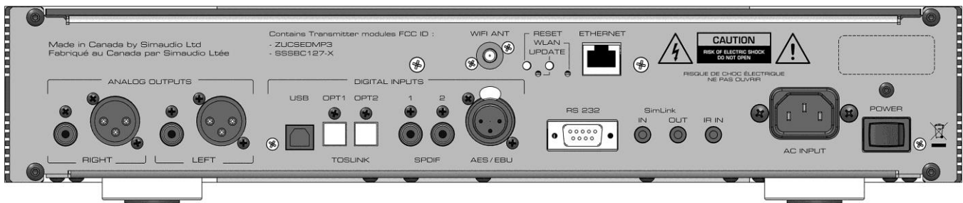
Figure 2: MOON 280D Rear panel
