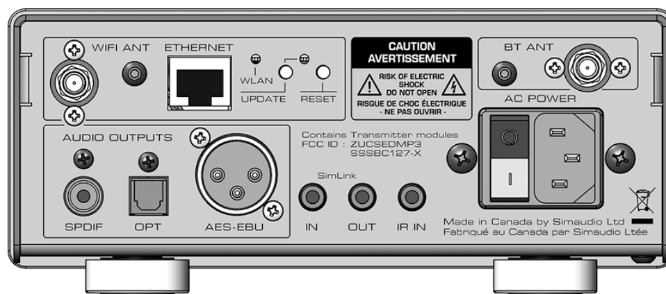
Figure 2: MiND 2 Rear panel
