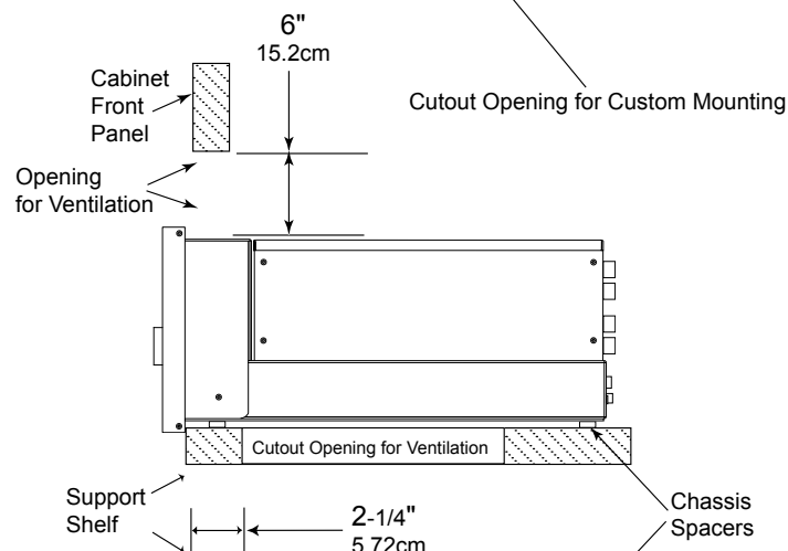
C2700 Side View in Custom Cabinet
