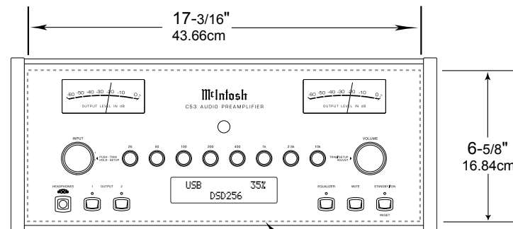
C53 Front Panel Custom Cabinet Cutout
