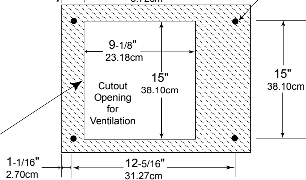
C53 Bottom View in Custom Cabinet
