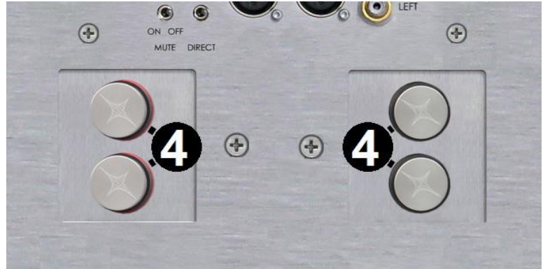
Hercules II Mono binding post layout
