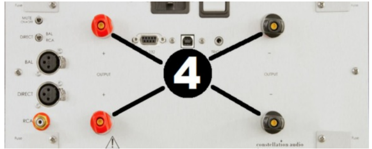
Taurus Mono binding posts
