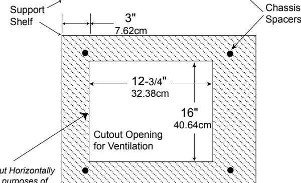
MC312 Bottom View in Custom Cabinet
