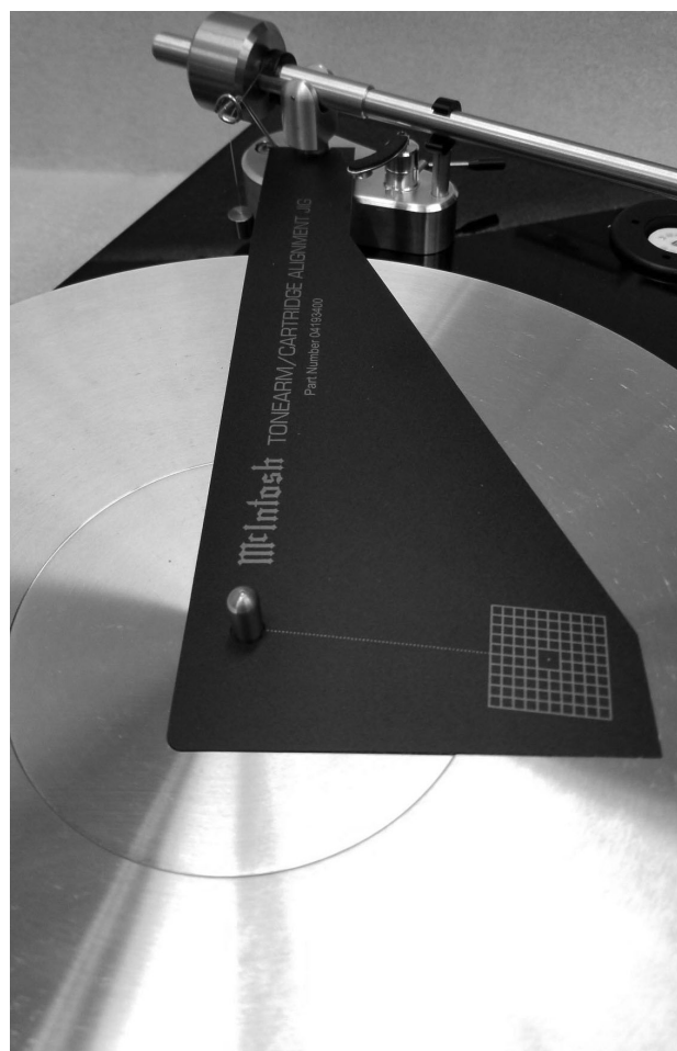
Figure 14— Alignment jig
