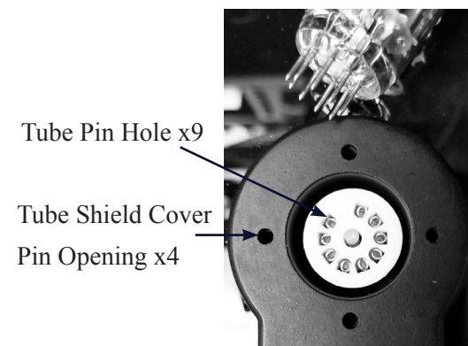
Figure 02– Tube Socket
