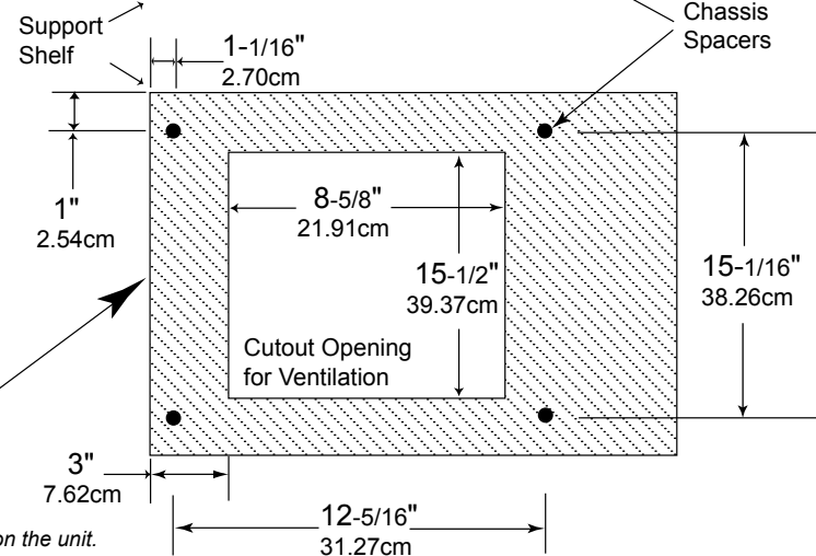
MCT500 Bottom View in Custom Cabinet
