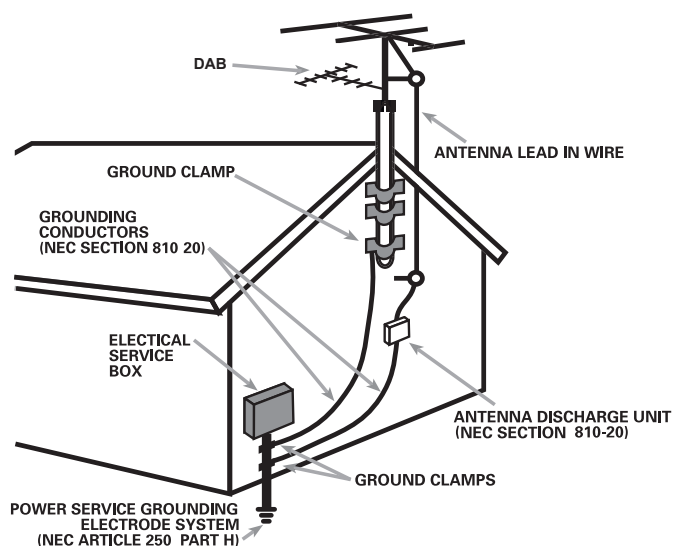
ANTENNA GROUNDING ACCORDING TO NATIONAL ELECTRICAL CODE INSTRUCTIONS SECTION 810: "RADIO AND TELEVISION EQUIPMENT"
