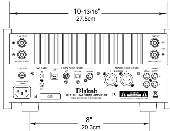
Rear View of the MHA150
