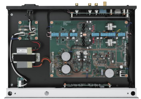
Internal configuration
