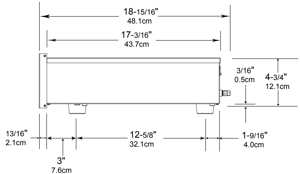
Side View of the MC301
