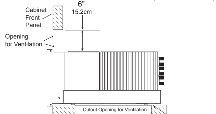
MC8207 Side View in Custom Cabinet
