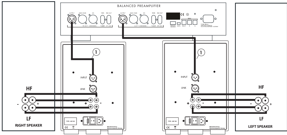
1: Standard XLR cable
