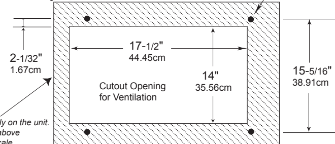
MC2301 Bottom View in Custom Cabinet
