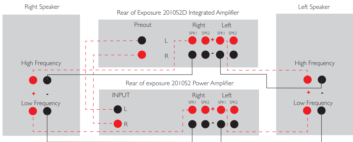
Connecting a pair of loudspeakers in bi-wiring mode
